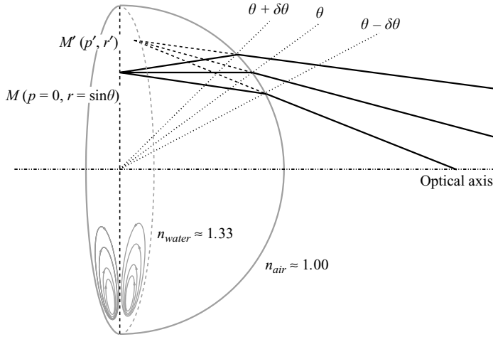
FIGURE 6. Schematic ray-tracing diagram of the geometrical optics for a spherical liquid lens.
