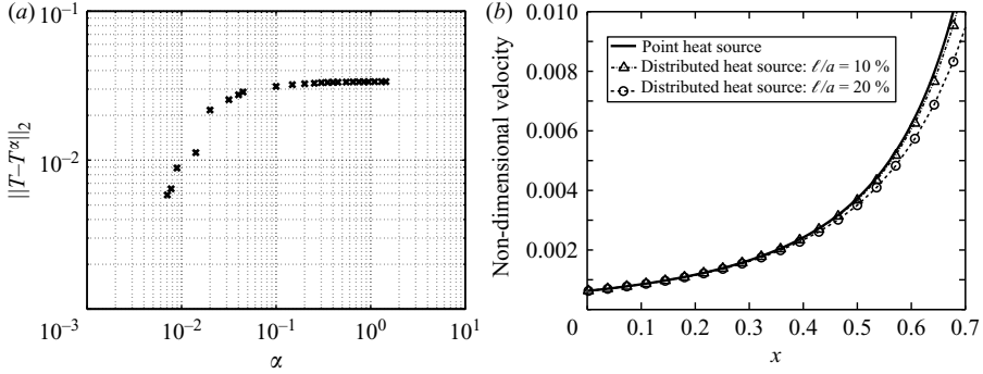
FIGURE 9. (a) Error \|T - T^\alpha\|_2 as a function of \alpha showing the convergence of the sequence T^\alpha to the point heat source solution T . (b) Velocity profile |\mathbf{u}| along the x -axis for the point heat source solution and for distributed heat source solutions with \ell/a = 10\% and 20\% .
