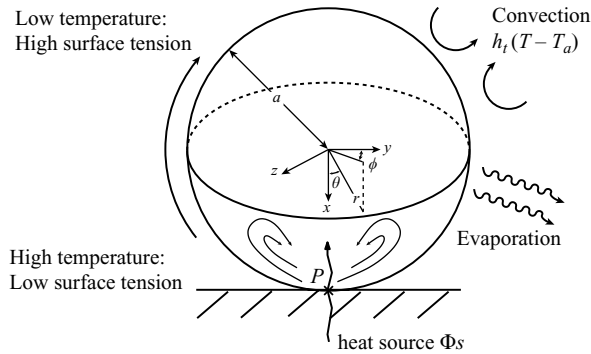
FIGURE 1. Schematic illustration and notation for a droplet on a superhydrophobic surface.
