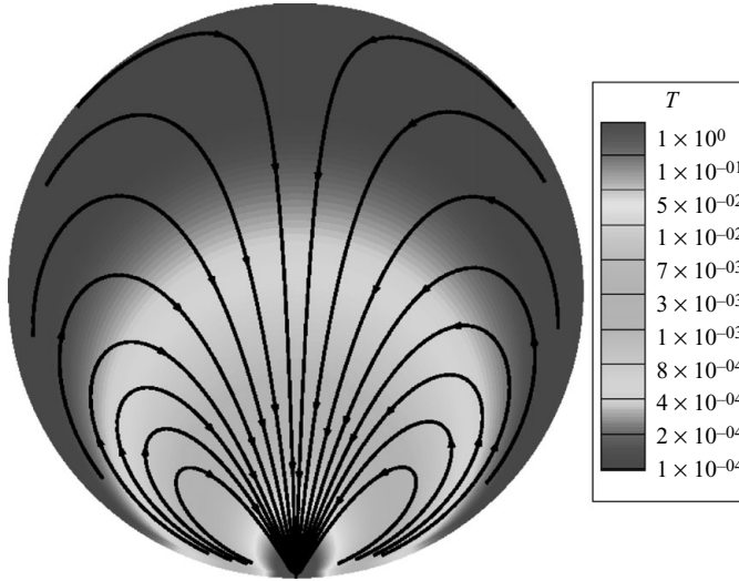
FIGURE 5. Analytic solution of the temperature field and corresponding streamlines. The colormap represents the dimensionless analytical temperature field for Bi = 800 and the black arrows represent the streamlines of the flow in the centreplane defined by \varphi = 0 . The analytical solution is computed using n = 100 terms in the expansion.
