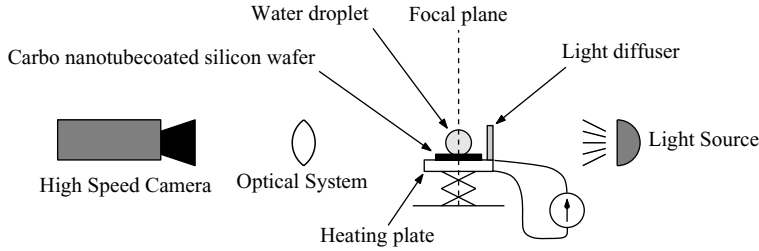
FIGURE 2. Schematic illustration of the experimental setup.
