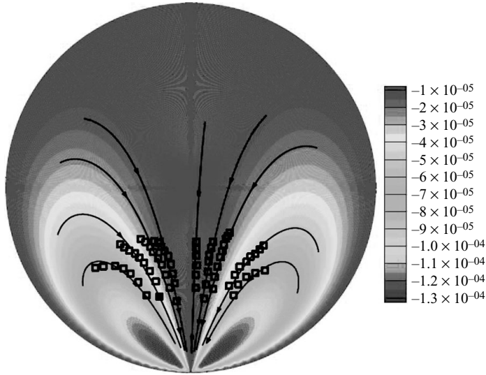
FIGURE 8. Analytic and experimental streamlines. The colormap represents the analytic streamfunction; black lines represent particular streamlines computed analytically; black squares represent experimentally recorded particle trajectories. The analytical solution is computed using n = 100 terms in the expansion.
