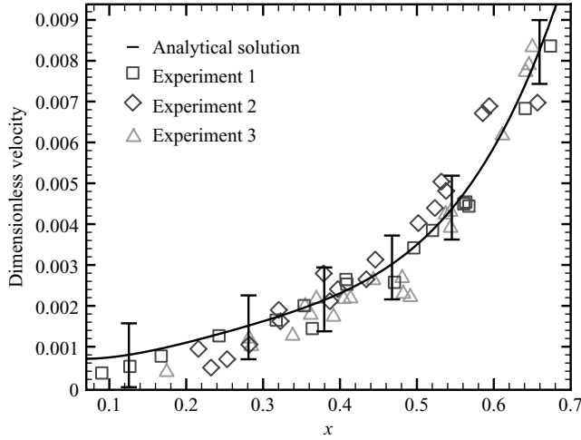
FIGURE 7. Analytic and experimental velocity profile, |\mathbf{u}| . The spatial variable x represents the dimensionless coordinate along the x -axis: x = 0 lies at the centre of the droplet, x = 1 lies at the contact point. The black line represents the analytic velocity profile in the drop for Bi = 800 . Different symbols correspond to three sets of data with heat sources of different intensity. Error bars give an estimate of the error in measuring the velocity of a particle by extracting the position of its centroid in successive frames and hence are a reflection of the resolution of the image.
