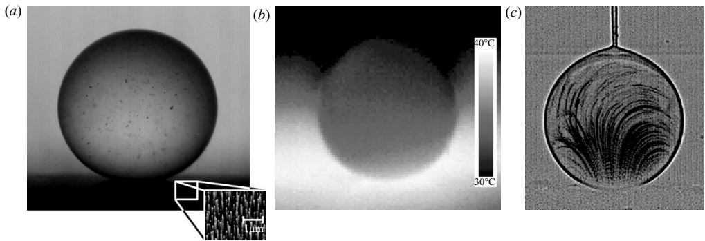
FIGURE 3. (a) Photo of a water droplet (0.5 mm radius) on a superhydrophobic surface seeded with silica tracer particles. The inset shows an SEM image of the surface coated with a carbon nanotube forest. (b) Thermal image of a drop deposited on the heated substrate showing contours of constant temperature. (c) Superposition of 20 consecutive snapshots of the water droplet taken at 10 ms time intervals, showing the inner convective motion of the fluid. Particles are moving downwards in the centre of the droplet. The ‘stem’ at the top of the droplet is the glass capillary that was used to deposit the droplet. The capillary was removed before any data was recorded. It bears emphasis that for illustration purposes, images (b) and (c) were taken using larger values of heat flux and brighter lighting than those used in data collection. In subsequent experiments, the temperature at the heating plate was lowered in order to remain in the stable roll regime, and the light source was dimmed to avoid thermal contamination.
