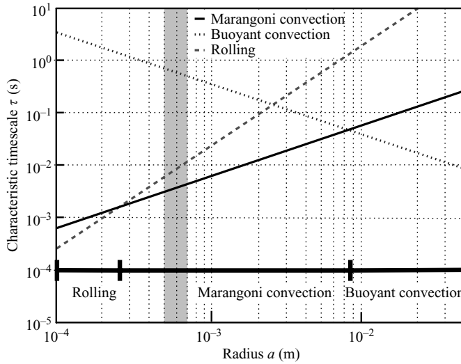
FIGURE 4. Characteristic convective time scales for various sizes of water droplets. The grey shaded region indicates the range of droplet sizes in our experiments. Material parameters correspond to those of water with \Delta T = 1^\circ\text{C} . Note that, as all three curves scale linearly with \Delta T , changing the temperature difference does not change the radius at which the curves intersect – rather it rescales the vertical axis.
